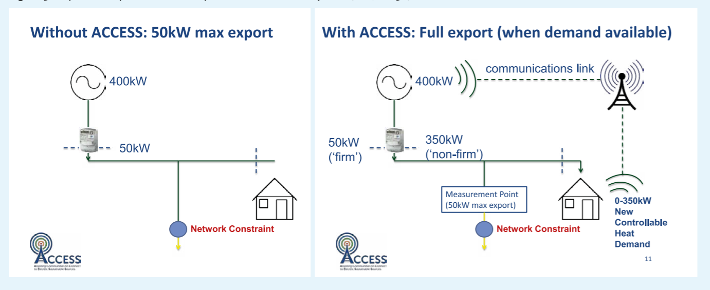
Figure 3: Before and after installation of the ACCESS network system (CES, 2015b)
