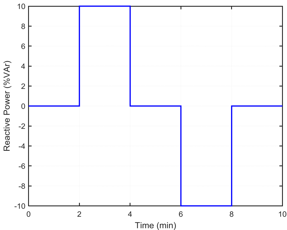
Fig. 4. Test Profile 2 – ESS reactive-power calibration test profile
