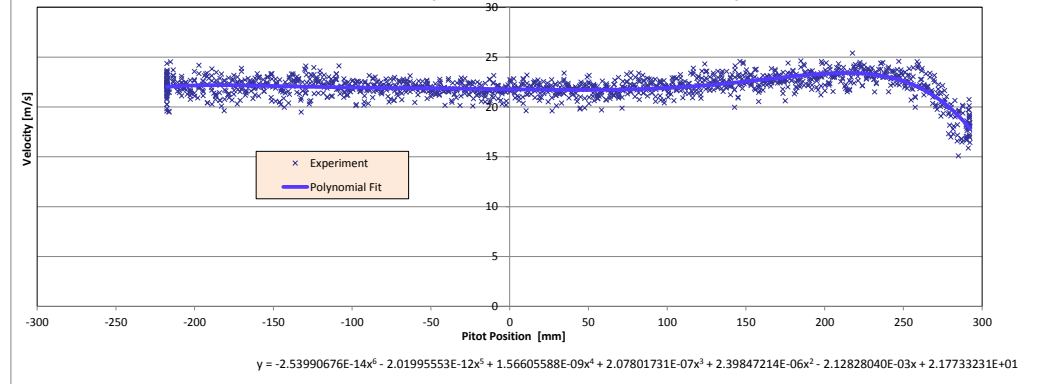
Raw Data Plot with Polynomial fit on Calculated Velocity
