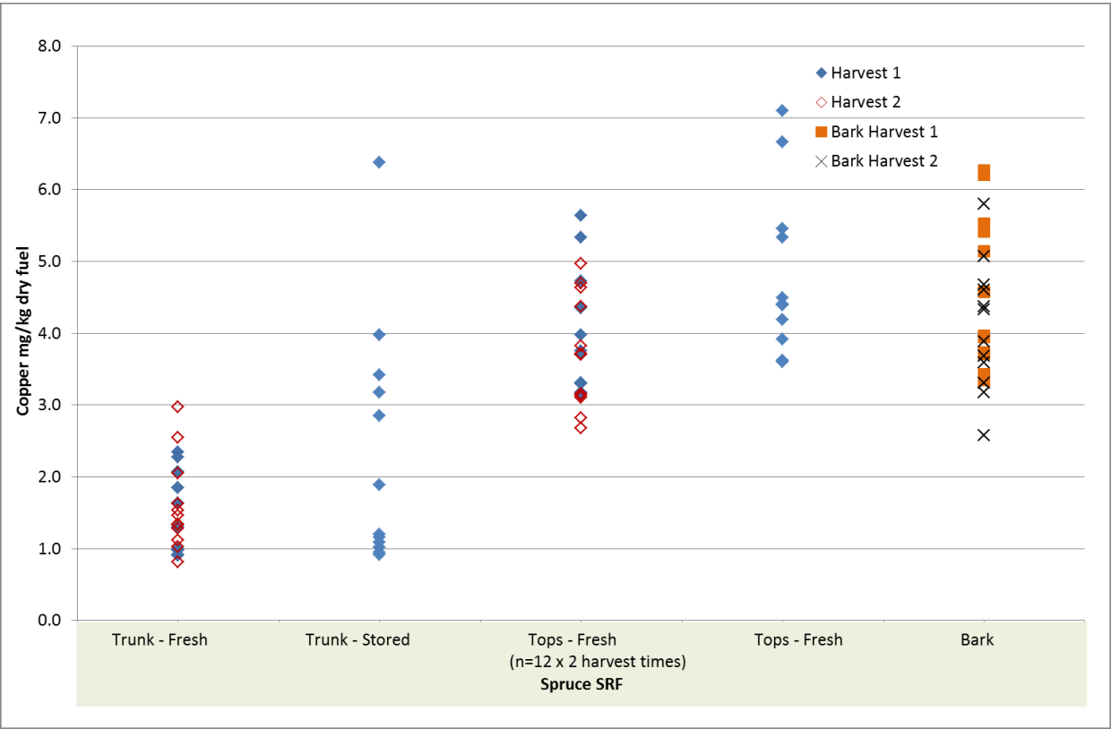
Copper content of Spruce SRF
