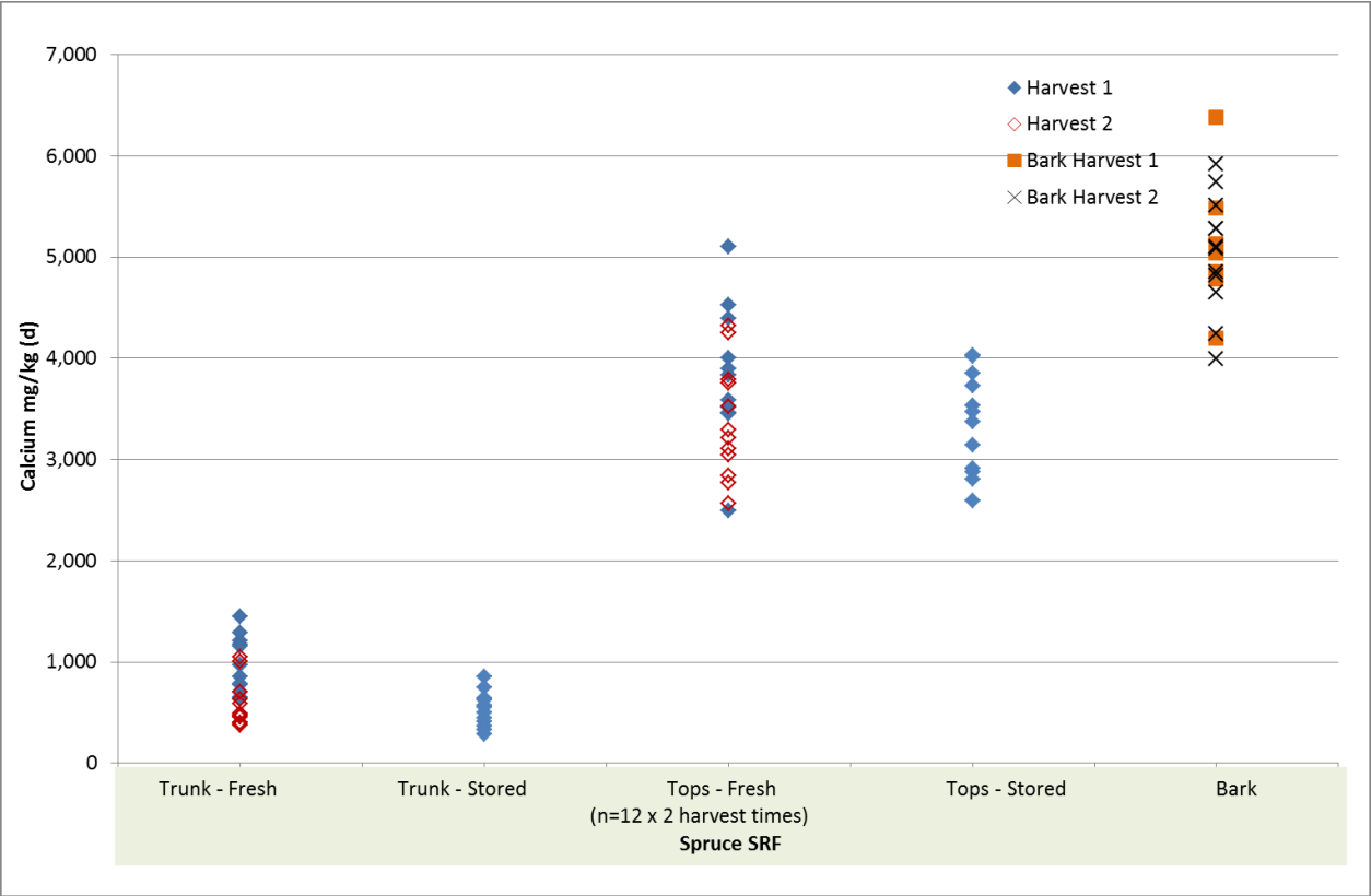
Calcium content of Spruce SRF
