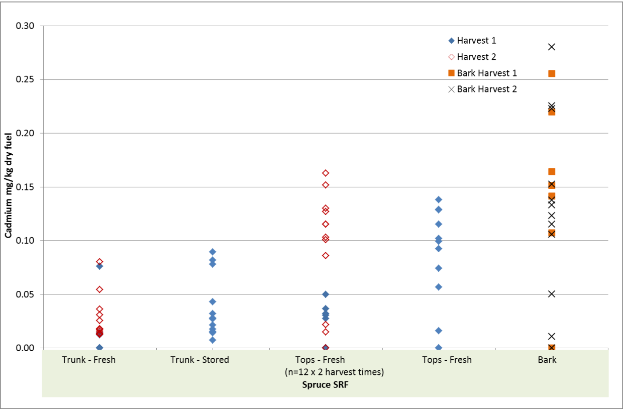
Cadmium content of Spruce SRF
